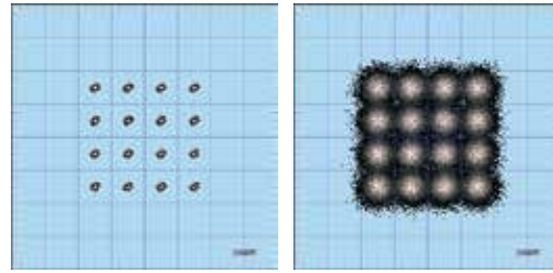
16QAM
