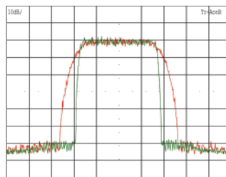
Sharp Carrier Roll-Off 8% versus 35%
