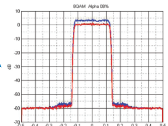
Example Smart Carries Bandwidth Savings of 50%
