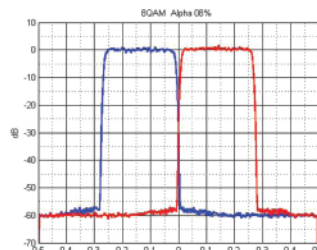
Example Smart Carries Bandwidth Savings of 50%
