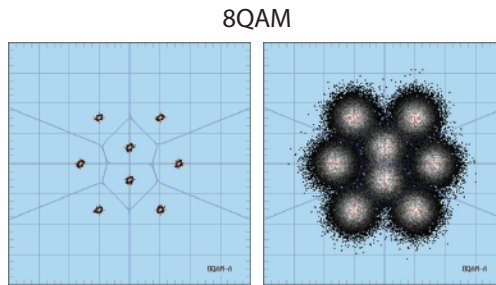
M7 Constellation monitor with and without noise
