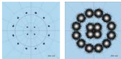
16APSK Constellation with and without Noise
