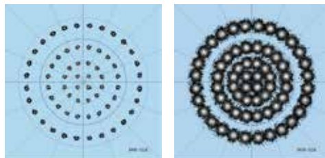
64APSK Constellation with and without Noise
